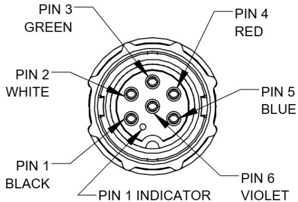
FRONT CONNECTOR END VIEW
