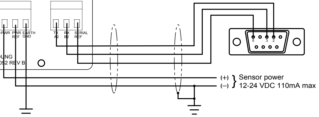
Typical DB-9 RS-232 Connection
